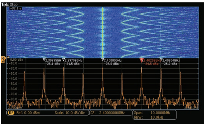
Figure 5. Spectrogram on an MDO3000.
