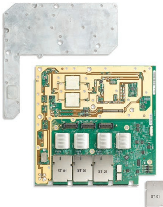
Figure 10. MDO4000C analog board with shields removed clearly shows the RF signal path.
