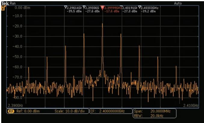
Figure 3. MDO3000 spectrum analyzer display elements.
