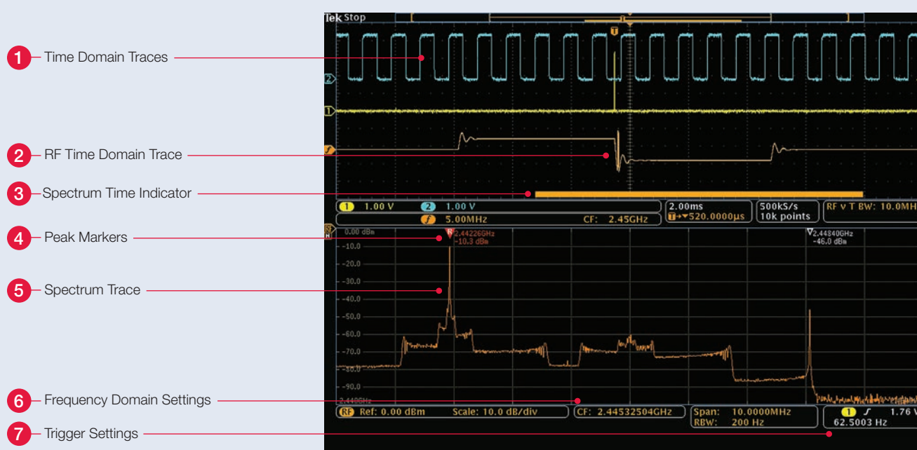
Figure 6. MDO4000 Series display elements.
