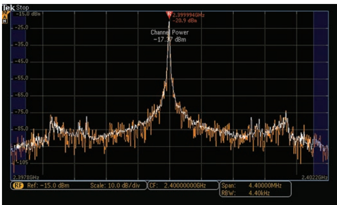
Figure 4. Channel power measurement on an MDO3000.
